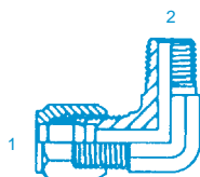
FL-2501 - 90° (1) Male Flareless (2) Male Pipe
