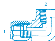
FL-2502 - 90° (1) Male Flareless (2) Fem. Pipe
