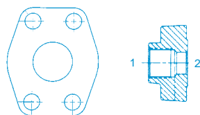
Y-SF-W104 (1) Fem. NPTF Thread (2) Flange - Tapped Holes Companion to Y-SF-W43K Code 61
