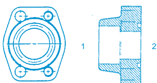
Y-SF-W43K (1) Fem. Pipe (2) Flange - with O-ring Groove Drilled Holes - O-Ring Kit Code 61
