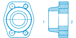
Y-SF-W3 (1) Deep Socket Weld Pipe (2) Flange - Tapped Holes Companion to Y-SF-W31K Code 61
