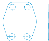
Y-SF-61-SP Shipping Plate Code 61
