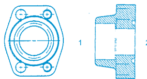
Y-SF-W44K (1) Fem. Pipe (2) Flange - with O-ring Groove Drilled Holes - O-Ring Kit Code 62
