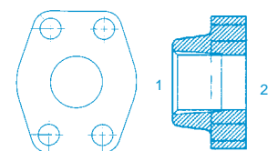
Y-SF-W45 (1) Fem. Pipe (2) Flange - Tapped Holes Companion to Y-SF-W44K Code 62
