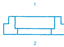
Y-SF-3301-61 (1) Braze (2) Flat Face Flange Code 61
