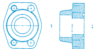
Y-SF-W31K (1) Deep Socket Weld Pipe (2) Flange with O-Ring Kit Drilled Holes Code 61
