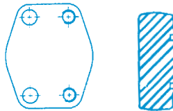
Y-SF-W36K Blanking Flange - with O-ring Groove Drilled Holes - O-Ring Kit Code 61
