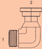
Y-OFS-1704-F-62 - 90°
