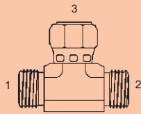
Y-OFS-6600-F - Tee (1) (2) Male OFS (3) Fem. OFS Swivel
