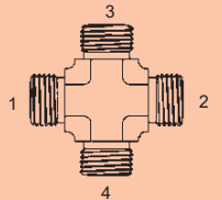
Y-OFS-2650-F - Cross (1) (2) (3) (4) Male OFS Union
