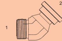
Y-OFS-1703-F-61 - 45° (1) Male OFS (2) O-Ring Flange Code 61
