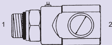
SLS-6805-SB-O - 90° (1) Male O-Ring - Stem (2) Fem. Pipe - Barrel (Short Body)
