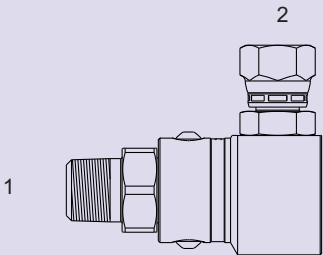
SLS-2573 - 90°
