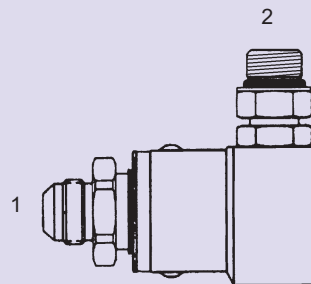
SLS-6814-5K-O - 90° 5000 PSI (1) Male JIC - Stem (2) Male O-Ring - Barrel
