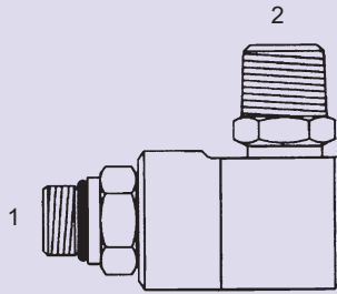
SLS-6806-O - 90° (1) Male O-Ring - Stem (2) Male Pipe - Barrel
