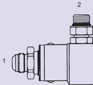
SLS-6814-4K-O - 90° 4000 PSI (1) Male JIC - Stem (2) Male O-Ring - Barrel
