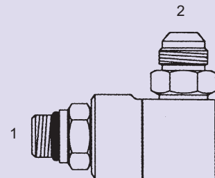
SLS-6841-4K-O - 90° 4000 PSI (1) Male O-Ring - Stem (2) Male JIC - Barrel
